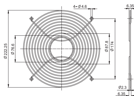
FG-25 For 254mm Fan
